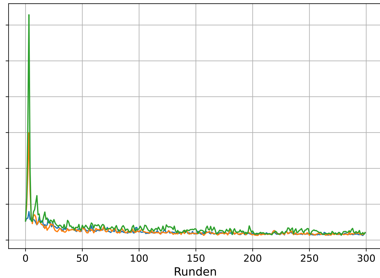
Starker Label Skew Loss
